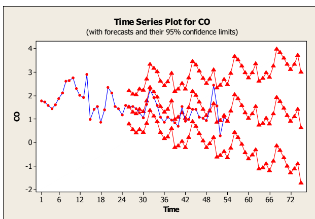
(a) CO
